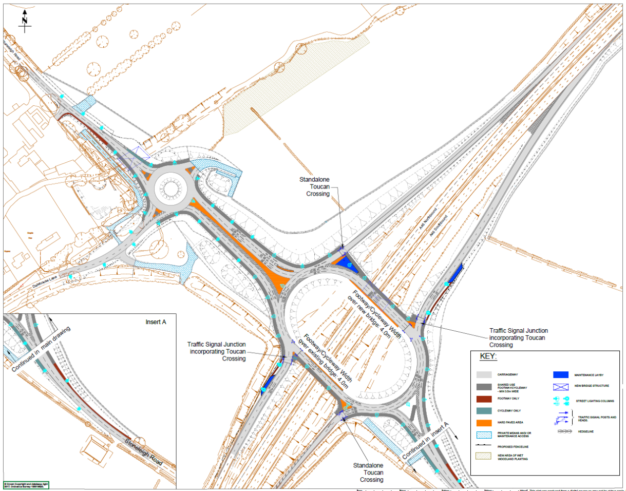
Figure 2: Proposed junction improvement scheme (Source: Warwickshire County Council)
