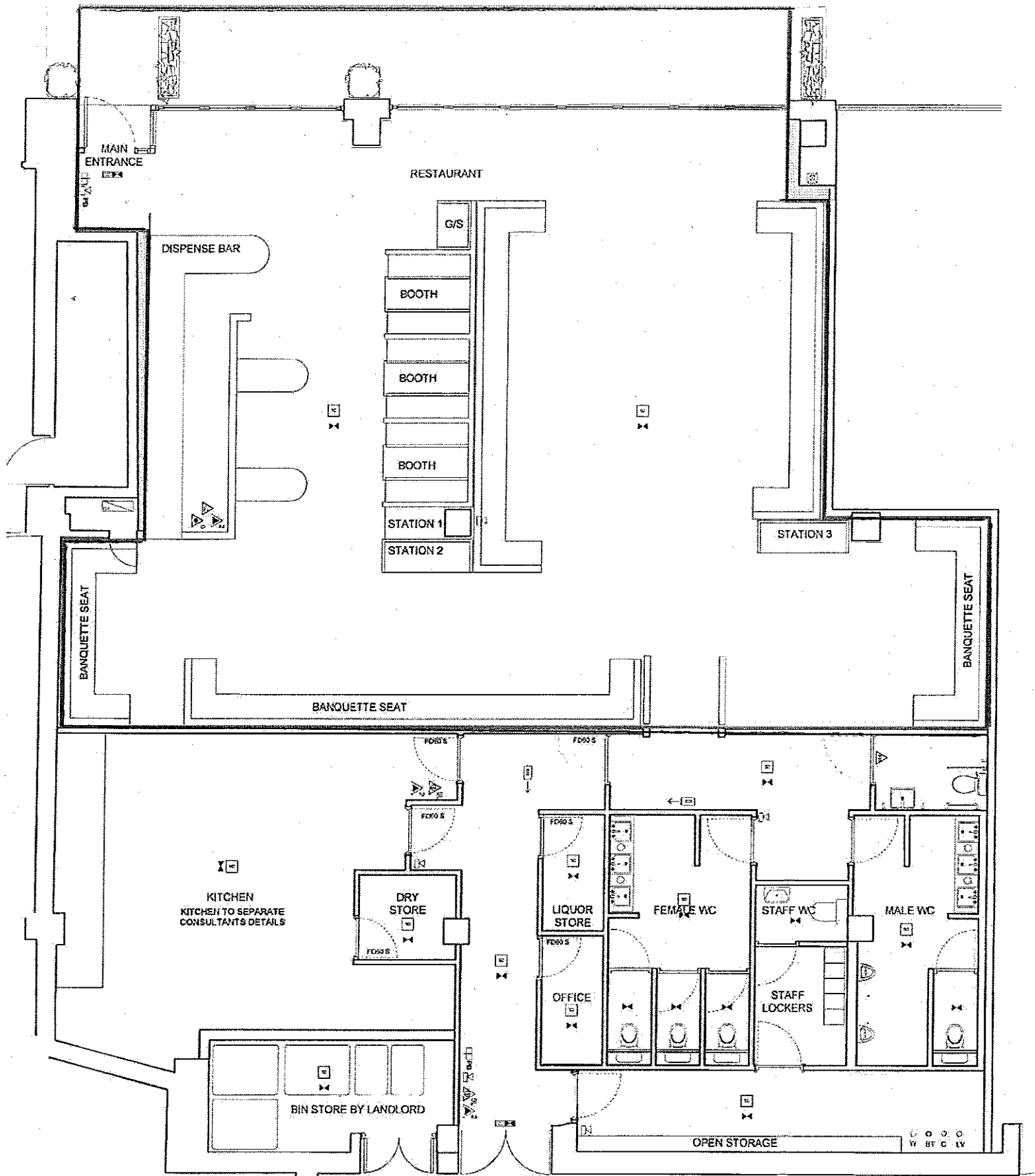
A GROUND FLOOR PLAN SCALE 1:50@A1
